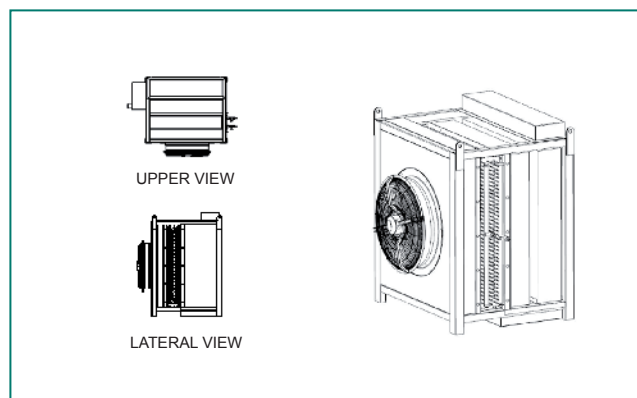
Design for models 1000 S.R. and 1500 S.R.
