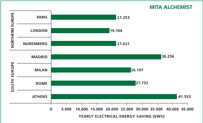
Simulation: Alchemist in a 160 kWf plant with parallel compression
