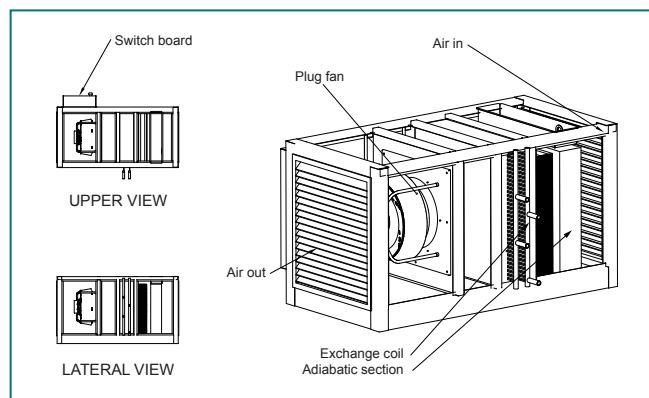
Design for models from 2500 S.R. to 5000 S.R.
