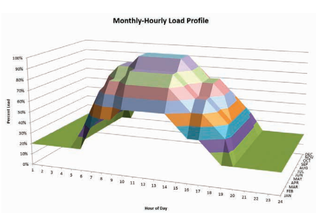
Fig. 3: Yearly HVAC load profile
